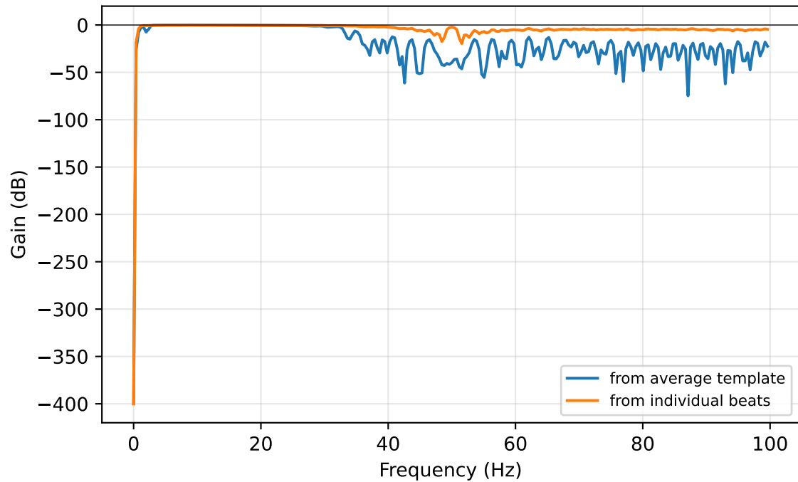
Resulting Wiener transfer function
